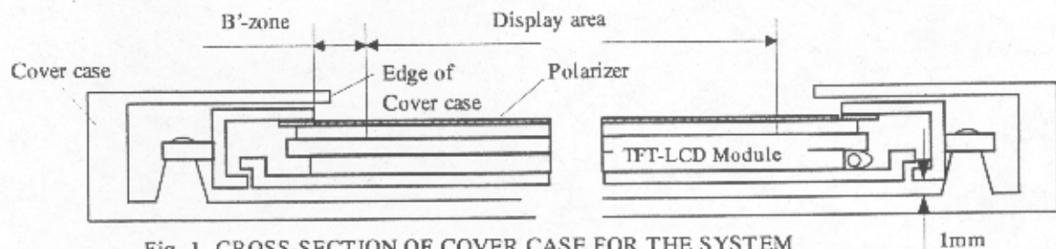
Fig. 1 CROSS-SECTION OF COVER CASE FOR THE SYSTEM
